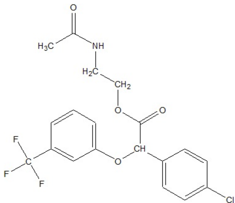
4-Chloro- \alpha -(3-(trifluoromethyl)phenoxy)benzeneacetic acid 2-(acetylamino)ethyl ester
